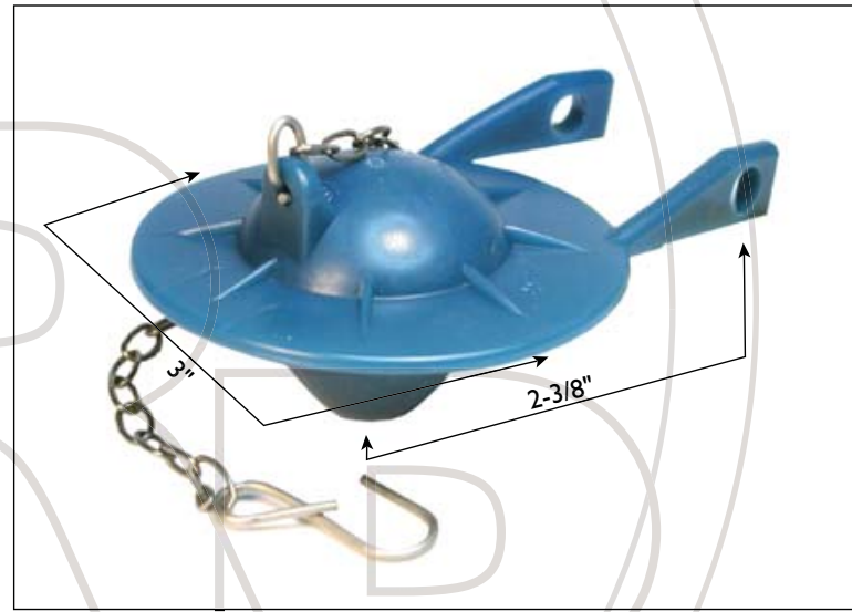
TUH113 • FLAPPER CHAIN: LINK W/ J-CLIP • CHAIN LENGTH: 8.5"
