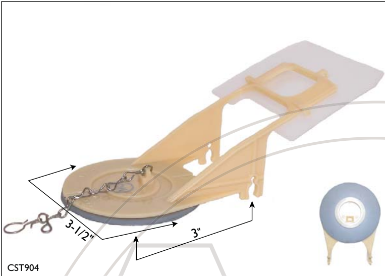
TUH092-5 • FLAPPER CHAIN: LINK W/ J-CLIP • CHAIN LENGTH: 3"
