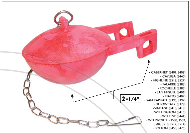
KOH49114 • FLAPPER CHAIN: LINK W/CLIP • CHAIN LENGTH: 8"
