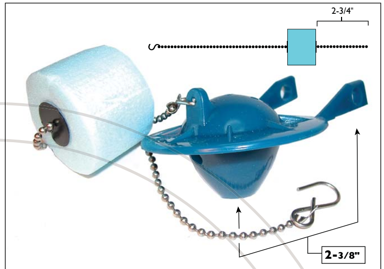
KOHGP85160 • FLAPPER CHAIN: BEADED W/J-CLIP • CHAIN LENGTH: 12" • FLOAT
