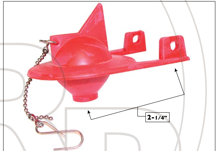
KOHGP89825 • FLAPPER CHAIN: BEADED W/J-CLIP • CHAIN LENGTH: 4-1/2"
