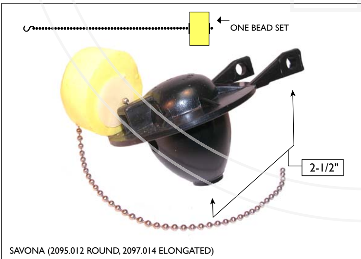
AMS738380 • FLAPPER 1 BEAD SET CHAIN: BEADED NO CLIP • CHAIN LENGTH: 9"
