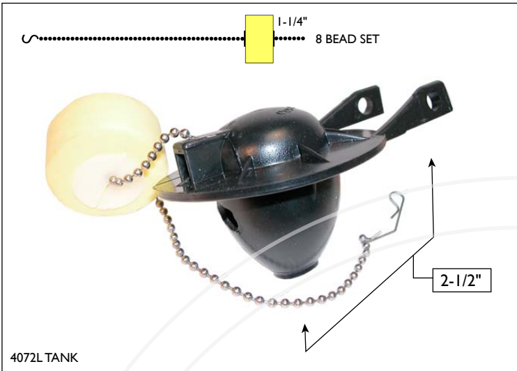
AMS738397 • FLAPPER 8 BEAD SET CHAIN: BEADED W/CLIP • CHAIN LENGTH: 9"
