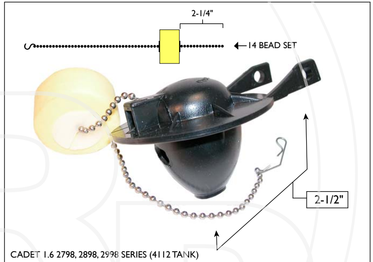
AMS738358 • FLAPPER 14 BEAD SET CHAIN: BEADED W/CLIP • CHAIN LENGTH: 9"
