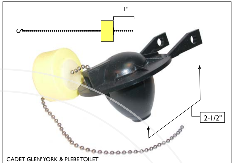
AMS738165 • FLAPPER CHAIN: BEADED NO CLIP • CHAIN LENGTH: 9"
