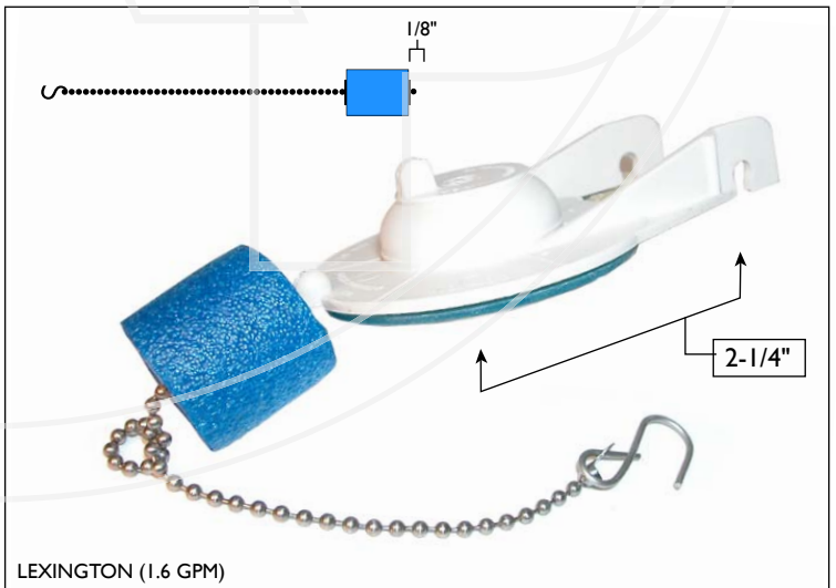
AMS738104 • FLAPPER CHAIN: LINK W/J-CLIP • CHAIN LENGTH: 8"
