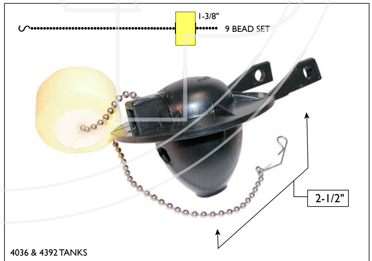
AMS738392 • FLAPPER 9 BEAD SET CHAIN: BEADED W/CLIP • CHAIN LENGTH: 9"
